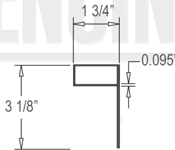
P Insert • 93" Length
