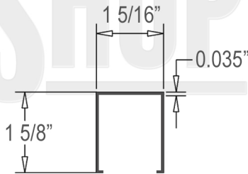
U Insert • 93" Length
