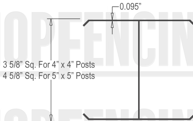
Post Insert • 72" Length For 4" Posts - 96" Length For 5" Posts
