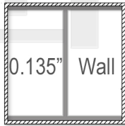
4" x 4" Posts
