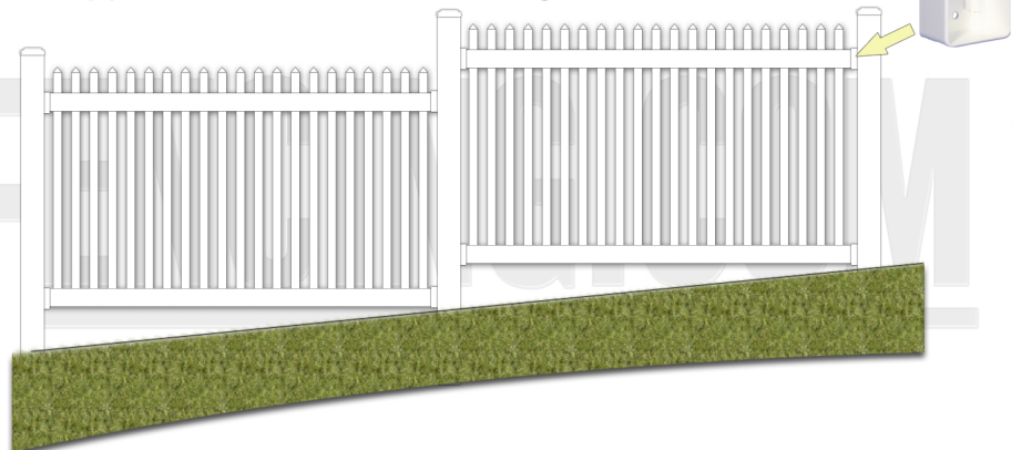
Stepped Panel Installation Using Wall Mounts
